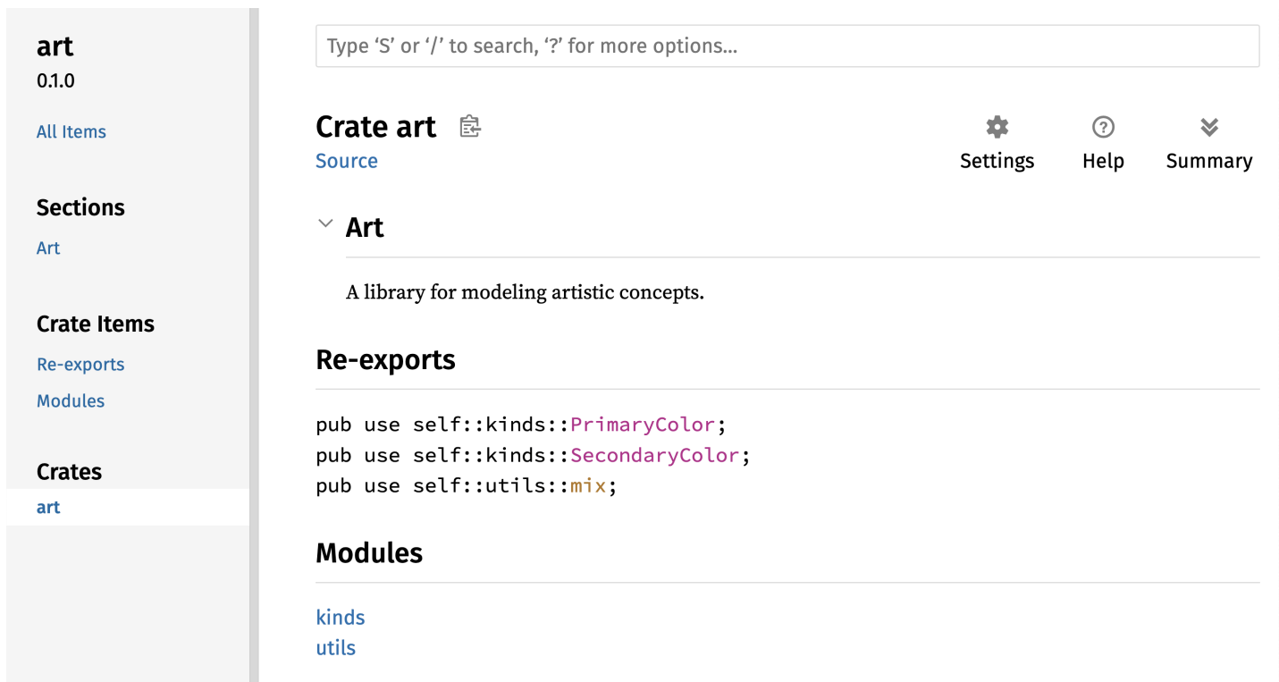
Figure 14-4: The front page of the documentation for art that lists the re-exports
